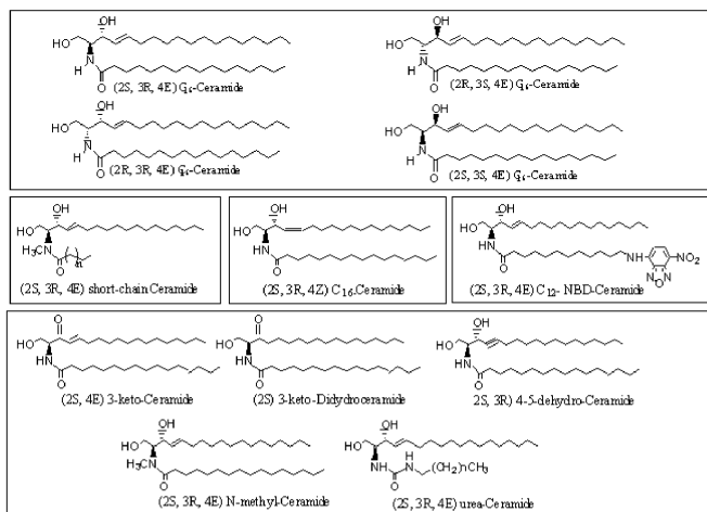
Fig. 2. Structures of synthetic ceramide analogs used in this study.
